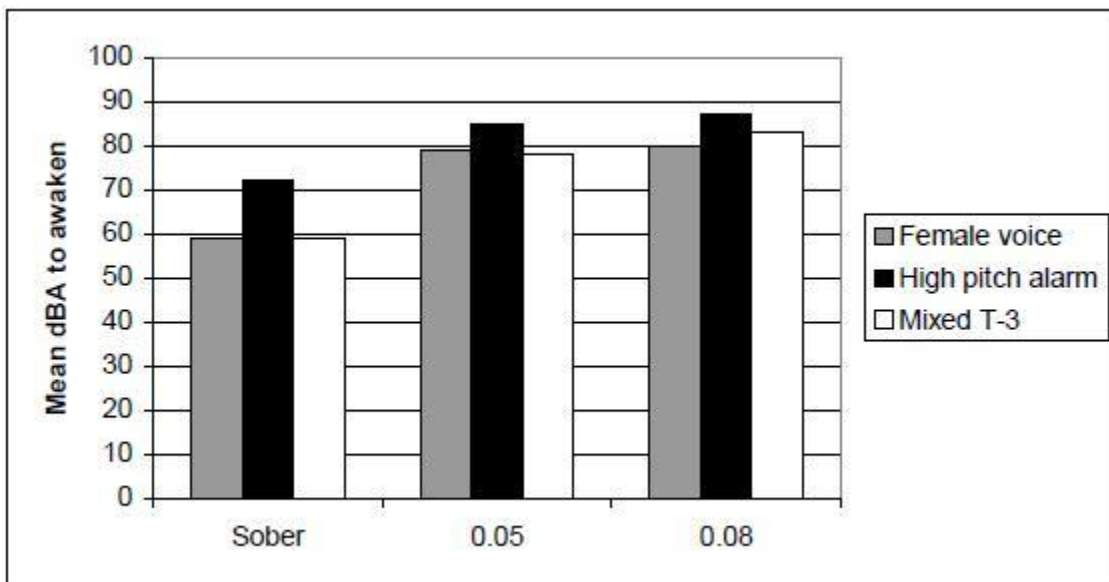
Figure 10: Mean Sound Level for Auditory Signals Required to Awaken Young Adults by Blood Alcohol Content ( Bruck et al., 2007 )
