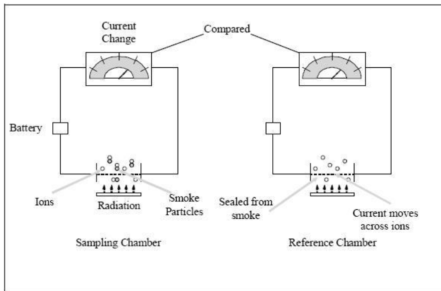
Figure 1: Representation of Ionization Smoke Detector ( O'Connor et al., 2008 )
