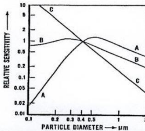
Figure 5: Relative Sensitivities of Detector Technologies vs. Particle Size (Bukowski, 1979)
