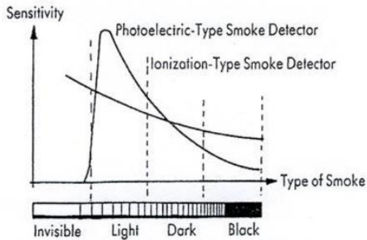
Figure 6: Response Sensitivity of Detectors vs. Smoke Color ( Bertschinger, 1988 )
