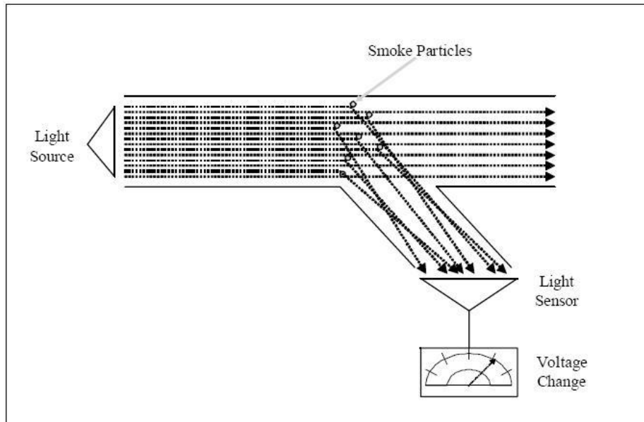
Figure 2: Representation of Photoelectric Smoke Detector (O'Connor et al., 2008)
