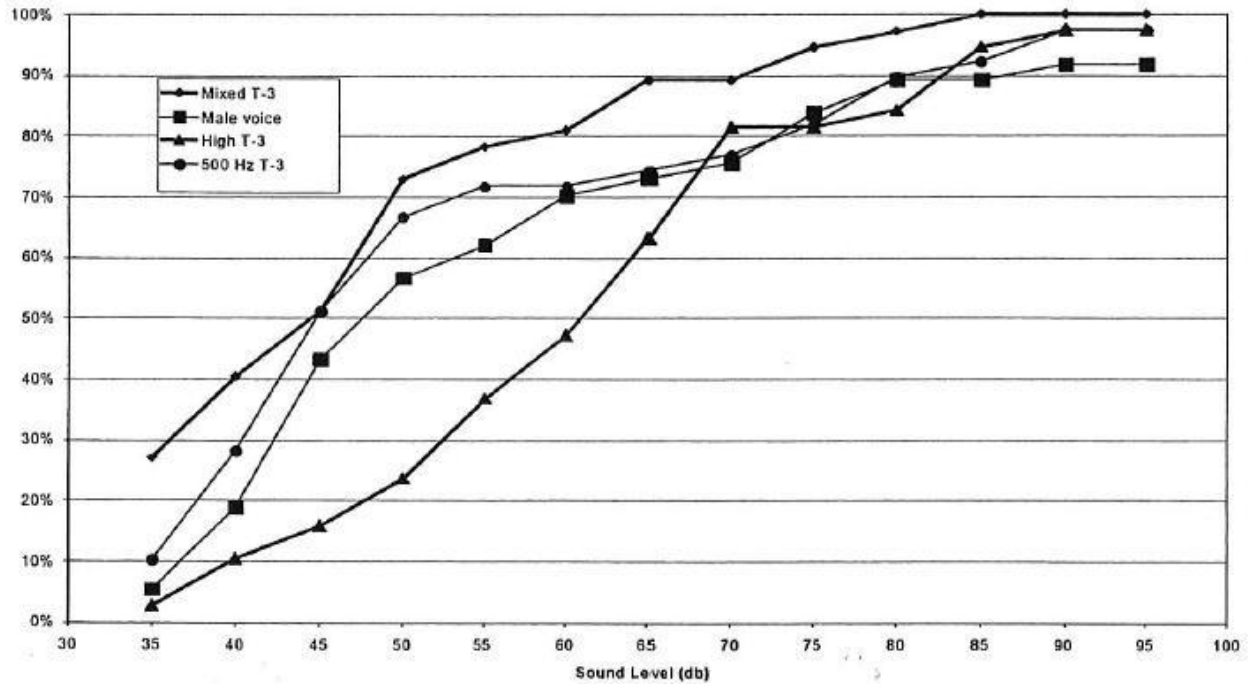
Figure 9: Percentage of Subjects who were Successfully Awakened by Signal Type and Sound Level (Bruck et al., 2006)
