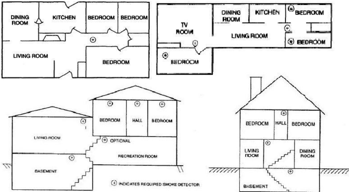
Figure 8: Possible Configurations for Residential Smoke Alarms (National Institute of Standards and Technology, 1995)
