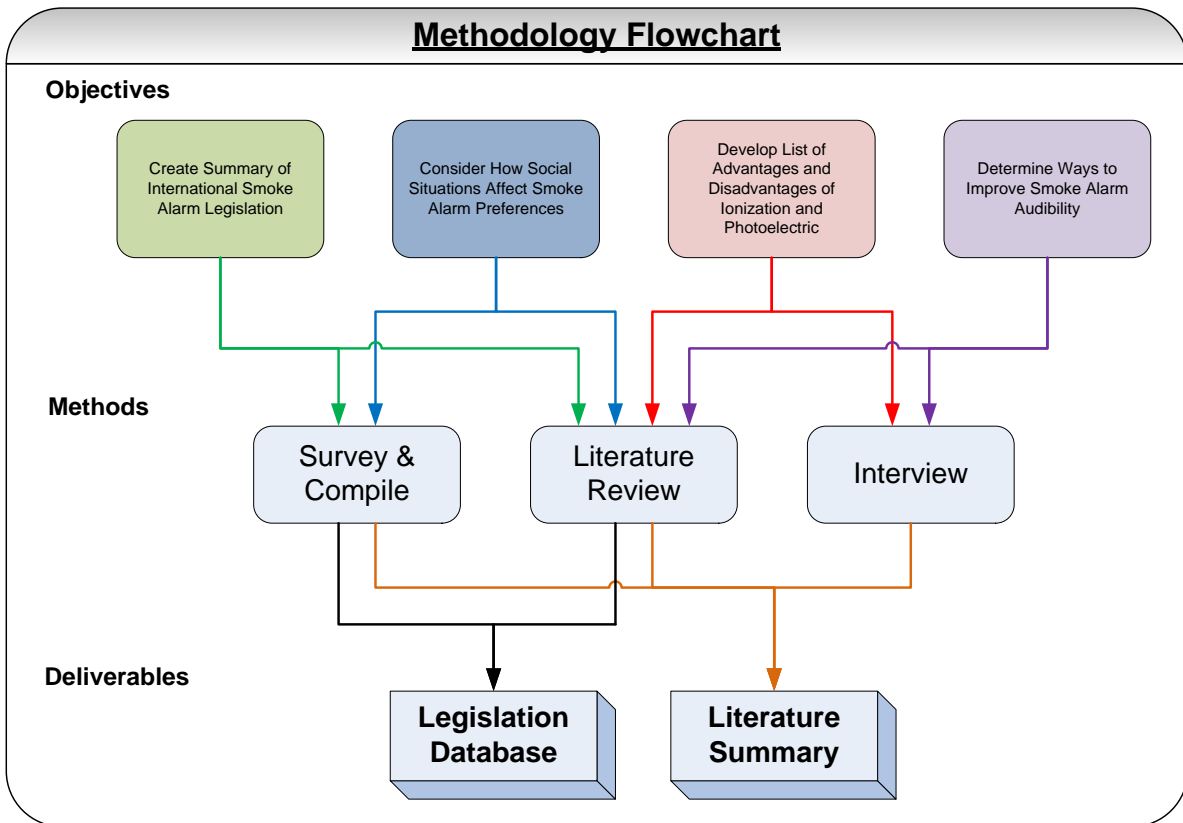
Figure 3: Methodology Flowchart
